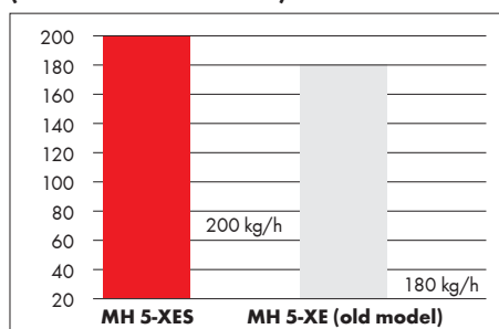
Chisel performance in kg/h (material: concrete B 35)
